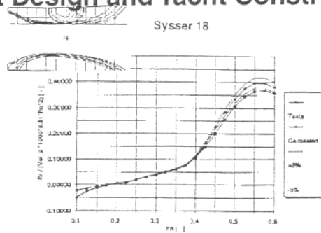
Figure 11: Comparison results model tests with expression 5 Sysser 18
