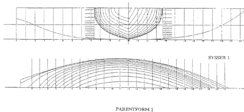
Figure 7: Parent 1 of series 1
