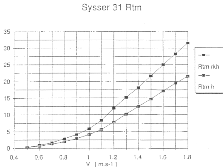
Figure 5: Comparison resistance with and without keel model of Sysser 31
