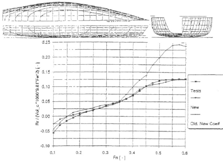
Figure 14: Comparison expression 5 with expression 3 and expression 4
