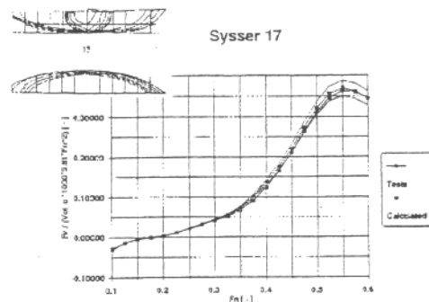
Figure 10: Comparison results model tests with expression 5 Sysser 17
