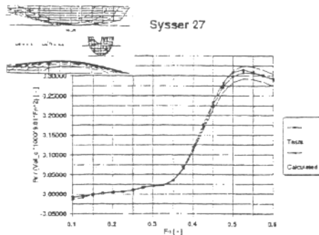
Figure 12: Comparison results model tests with expression 5 Sysser 27
