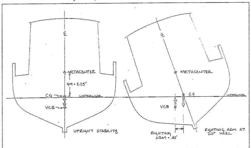
Stability terms. As the boat heels, VCB moves outboard of CG, creating a righting arm.
