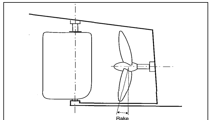
Figure 9 Blade rake
