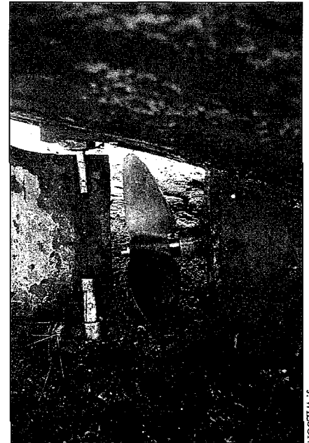
Photo 4 Very little clearance between hull and blade tip
