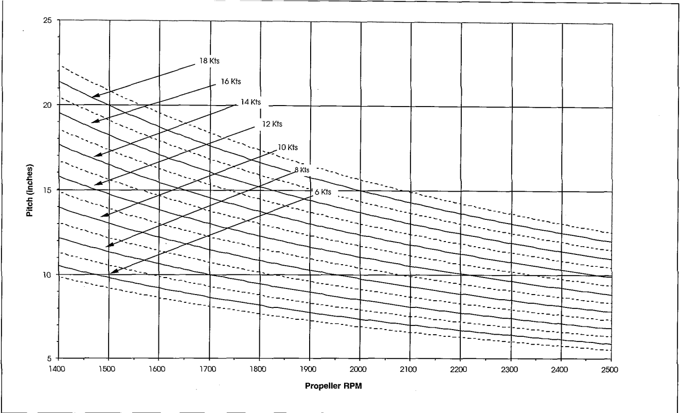
Figure 18 Propeller pitch chart (1 400-2 500 RPM)
