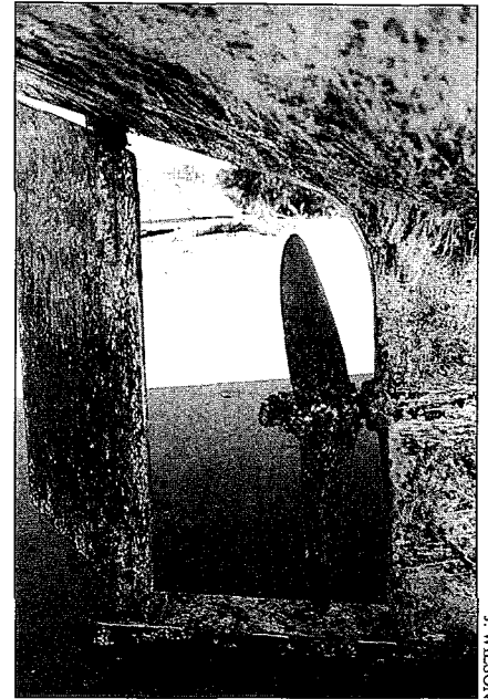
Photo 3 Too little clearance between deadwood and propeller
